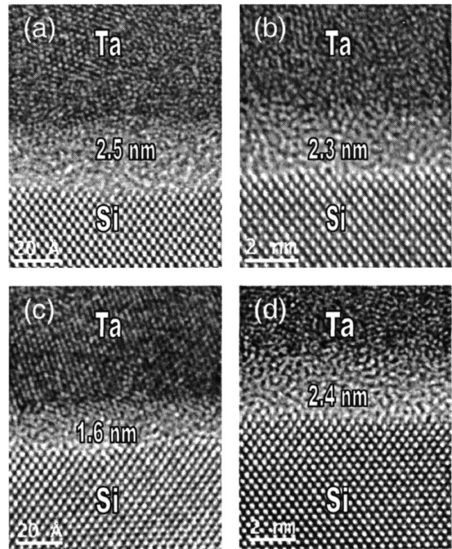
FIG. 2. TEM cross sections showing (a) as-deposited Ta/La_2O_3/SiO_2/Si gate stack and after reaction anneal of gate stacks at 400 °C in N_2 for (b) 10, (c) 20, and (d) 40 s. The amorphous dielectric thickness is indicated in each image.
