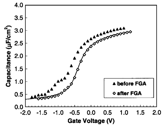
FIG. 6. Effects of a 400^\circ\text{C} , 20-min forming gas anneal on a lanthanum silicate dielectric stack; the data points show positive and negative V sweeps, the line a modeled fit (EOT 0.89 nm) to the data. The flatband voltage has shifted 0.23 V closer to the expected value (a reduction in positive charge density), and the “hump” related to the interface traps has been reduced. Capacitors are 50 \times 50 \mu\text{m}^2 , measured at 1 MHz.
