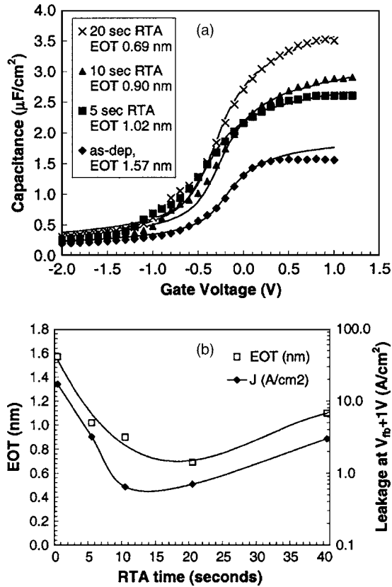
FIG. 1. (a) CV curves showing the effect of gate stack RTA time at 400 °C in N_2 ; the dots represent measured data and the lines modeled fits. (b) Corresponding plot of EOT (nm) and gate leakage J(A/cm^2) at V_{fb}+1V for the same devices. Dielectric reactions are evident from the changing stack EOT and J with RTA time. Capacitors are 71 \times 71 \mu m^2 , measured at 1 MHz.
