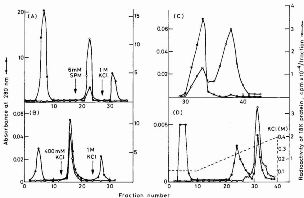
Fig. 1. Chromatography of radiolabeled hyp-18K protein on (A) Cibacron blue, (B) aminoocetyl-agarose, (C) Sepharose G-50 and (D) Mono Q columns, Conditions for chromatography are described in Materials and Methods.
