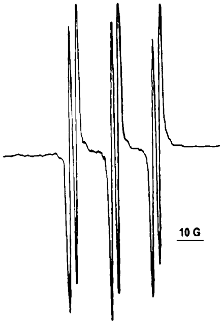
FIGURE 2 Hydroxyl radical formation by human osteoarthritic chondrocytes. EPR spectrum of primary human osteoarthritic chondrocytes ( 1 \times 10^6 /ml) in spin trapping reaction mixture of 4-POBN (10 mM), DTPA (0.1 mM) and ethanol (170 mM) in HBSS in the presence of exogenous ferrous sulfate (0.1 mM) with (B) or without (A) PMA-(100 ng/ml) stimulation. Instrument settings were: modulation amplitude, 1.0 G; time constant, 0.03 sec; scan rate 50 G/min; receiver gain, 4 \times 10^3 ; power, 10 mW. A representative experiment repeated twice.
